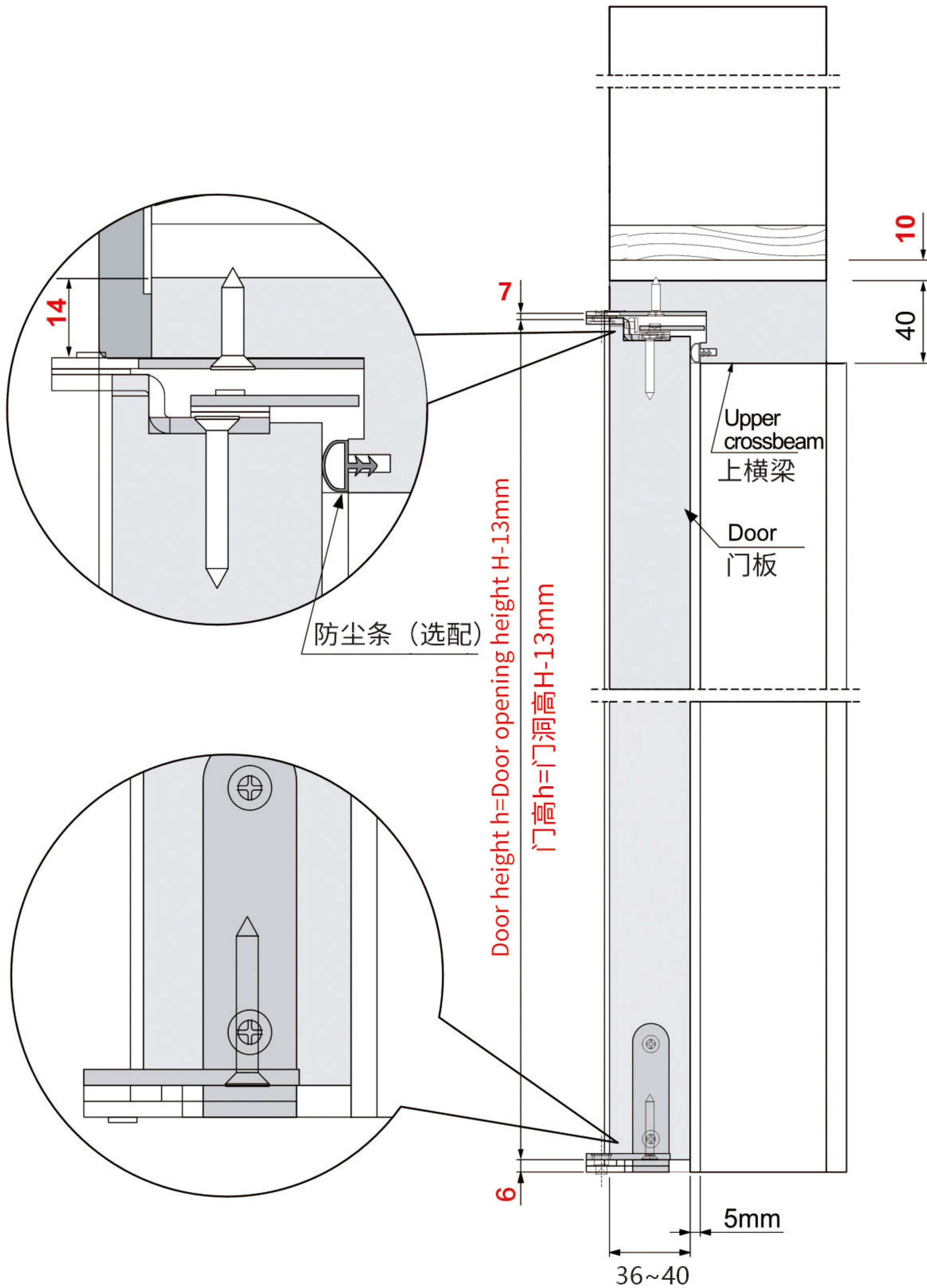
Vertical section (門框及門高參數圖)
