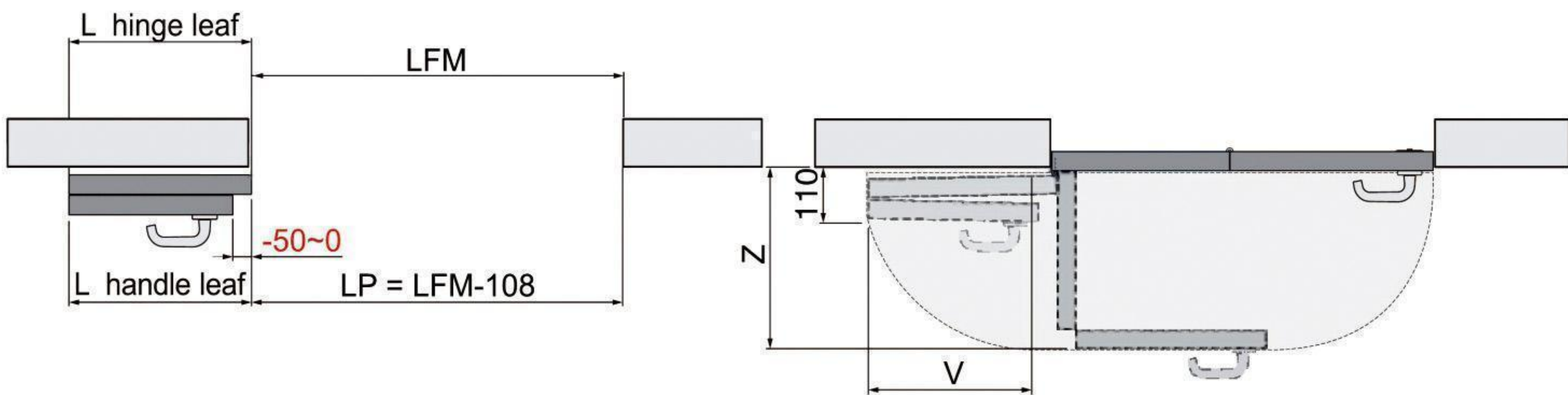
Dimensional diagram of the door-asymmetric leaves (不对等门尺寸图)
