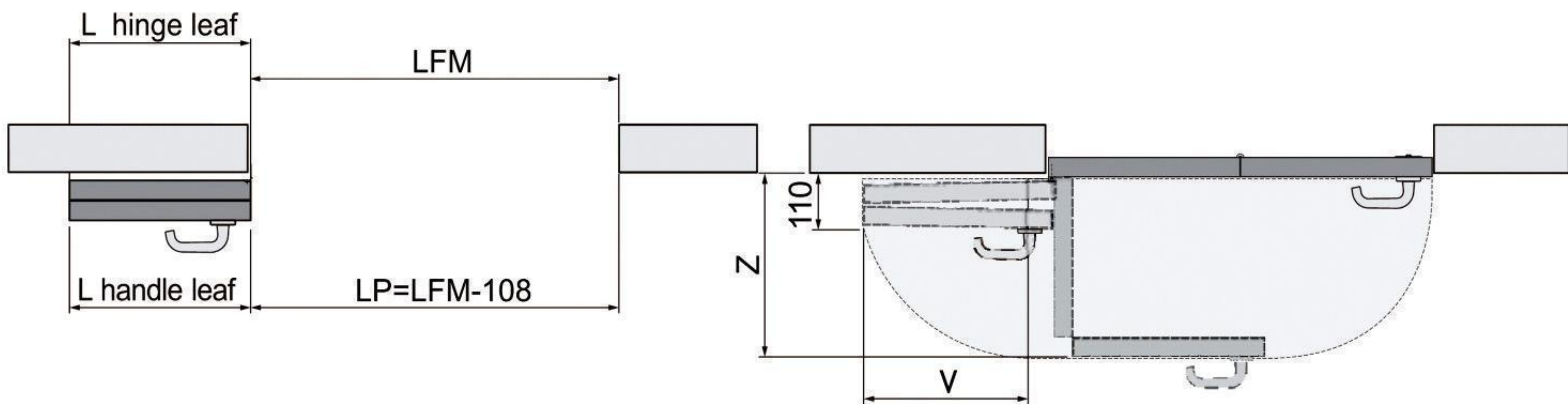
Dimensional diagram of the door-asymmetric leaves (不对等门尺寸图)
