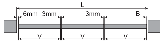
3 panels / 3扇门
