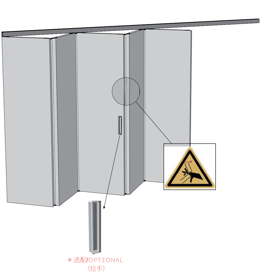
FIVE DOOR VERSION WITH SOFT-CLOSE / 五扇折叠门
