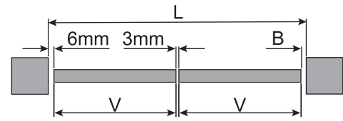
2 panels / 2扇门
